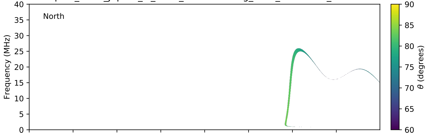
expres_earth_jupiter_io_isaac_lossc-wid1deg_3kev_20060104_v01.cdf
