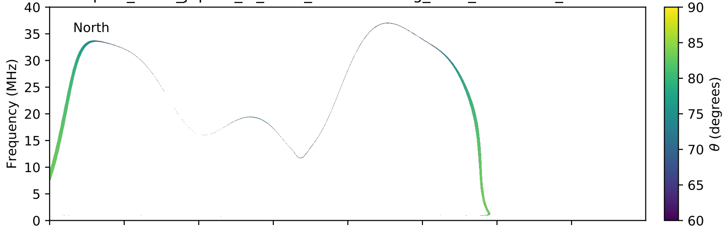
expres_earth_jupiter_io_isaac_lossc-wid1deg_3kev_20060103_v01.cdf
