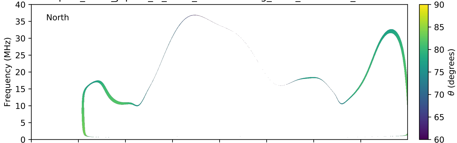
expres_earth_jupiter_io_isaac_lossc-wid1deg_3kev_20060101_v01.cdf
