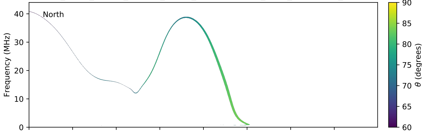
expres_earth_jupiter_europa_jrm09_lossc-wid1deg_3kev_20060131_v01.cdf
