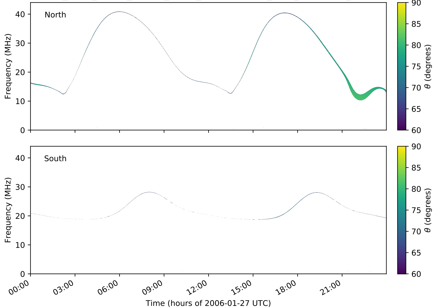
expres_earth_jupiter_europa_jrm09_lossc-wid1deg_3kev_20060127_v01.cdf
