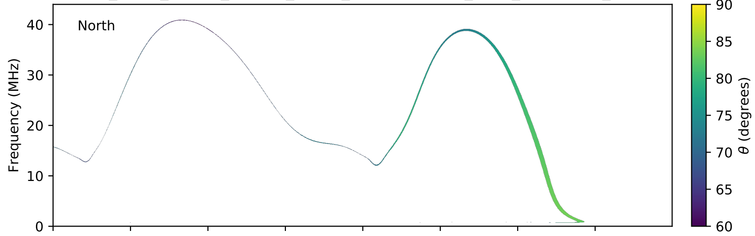
expres_earth_jupiter_europa_jrm09_lossc-wid1deg_3kev_20060113_v01.cdf
