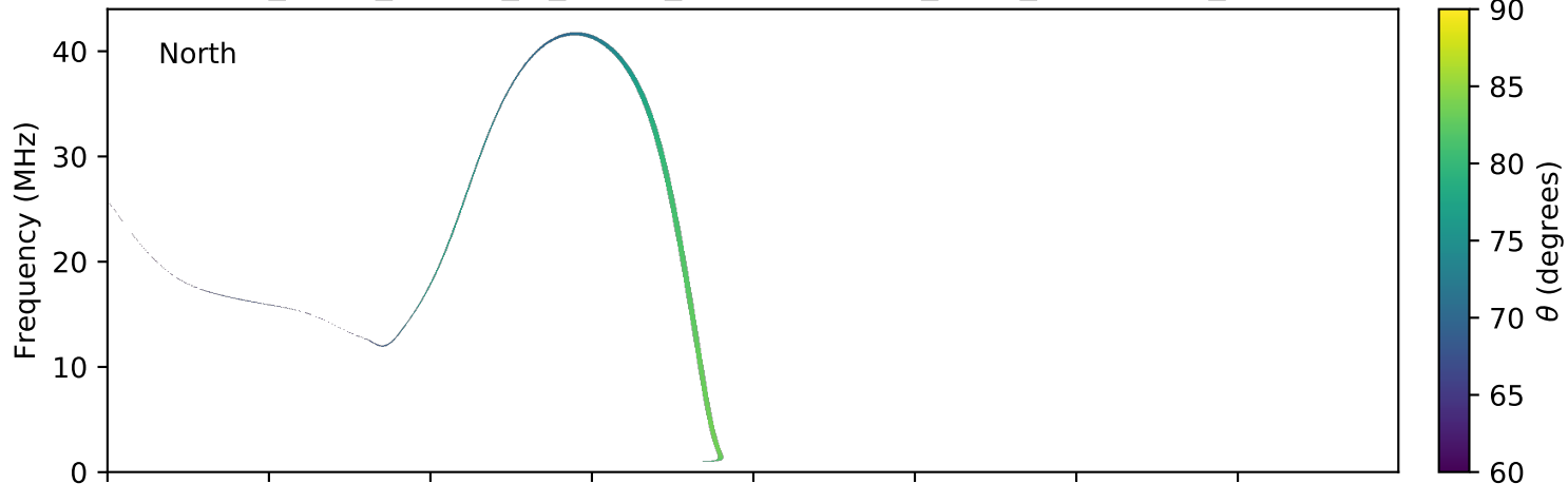
expres_earth_jupiter_io_jrm09_lossc-wid1deg_3kev_20051229_v01.cdf
