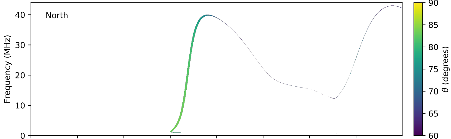
expres_earth_jupiter_io_jrm09_lossc-wid1deg_3kev_20051223_v01.cdf
