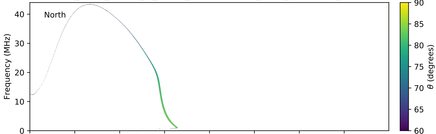
expres_earth_jupiter_io_jrm09_lossc-wid1deg_3kev_20051206_v01.cdf
