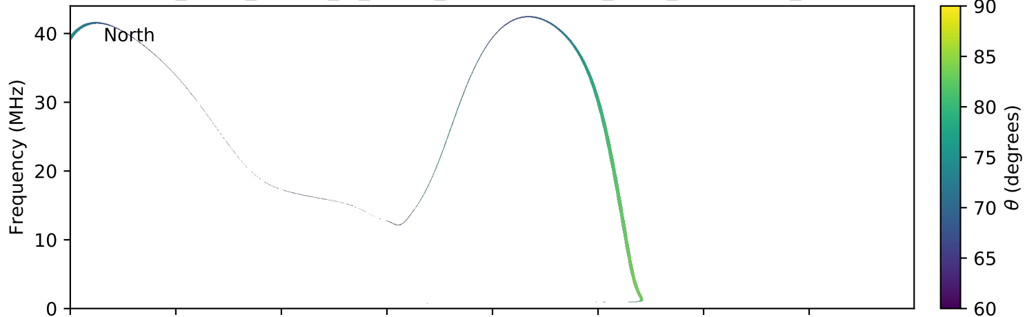
expres_earth_jupiter_io_jrm09_lossc-wid1deg_3kev_20051204_v01.cdf
