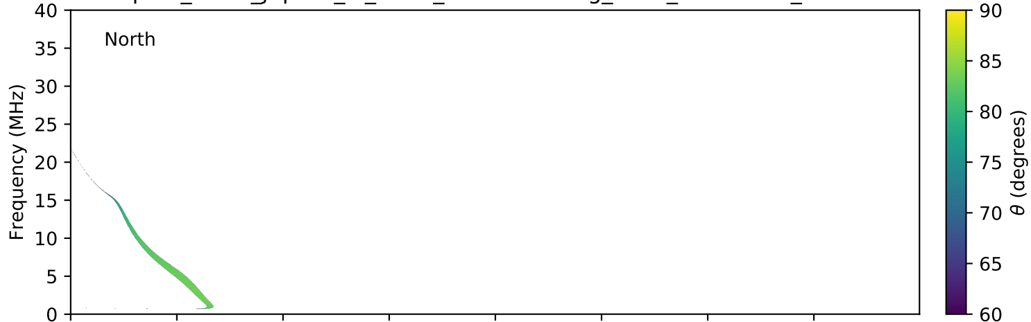
expres_earth_jupiter_io_isaac_lossc-wid1deg_3kev_20051231_v01.cdf
