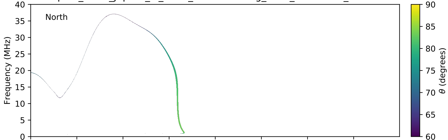
expres_earth_jupiter_io_isaac_lossc-wid1deg_3kev_20051229_v01.cdf
