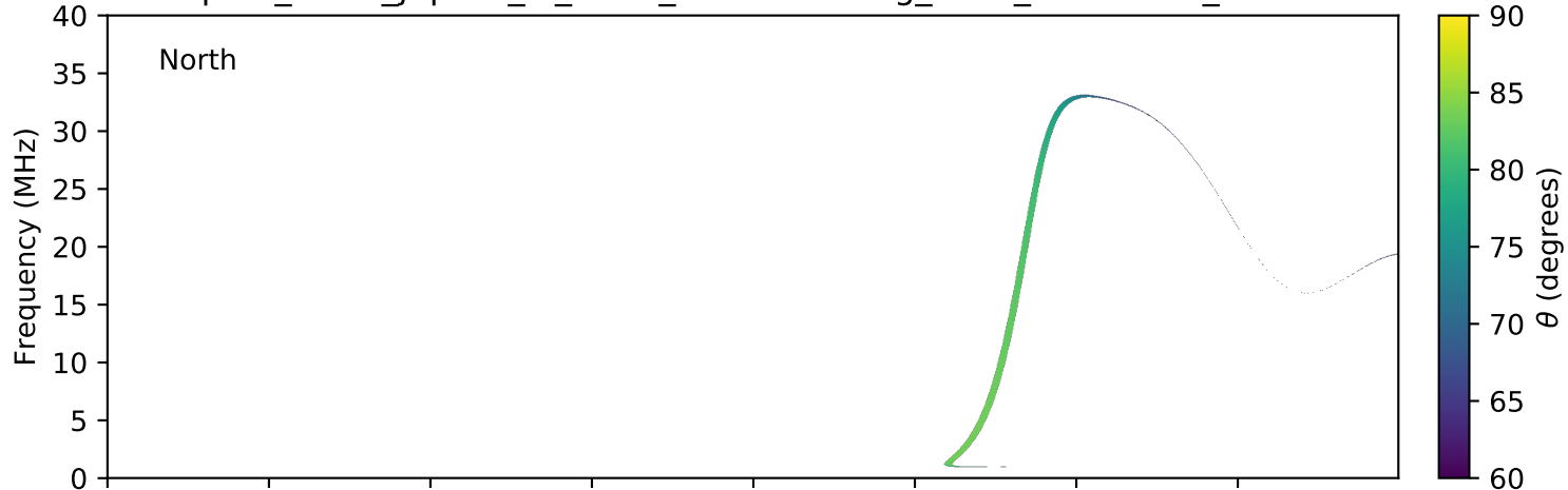
expres_earth_jupiter_io_isaac_lossc-wid1deg_3kev_20051228_v01.cdf
