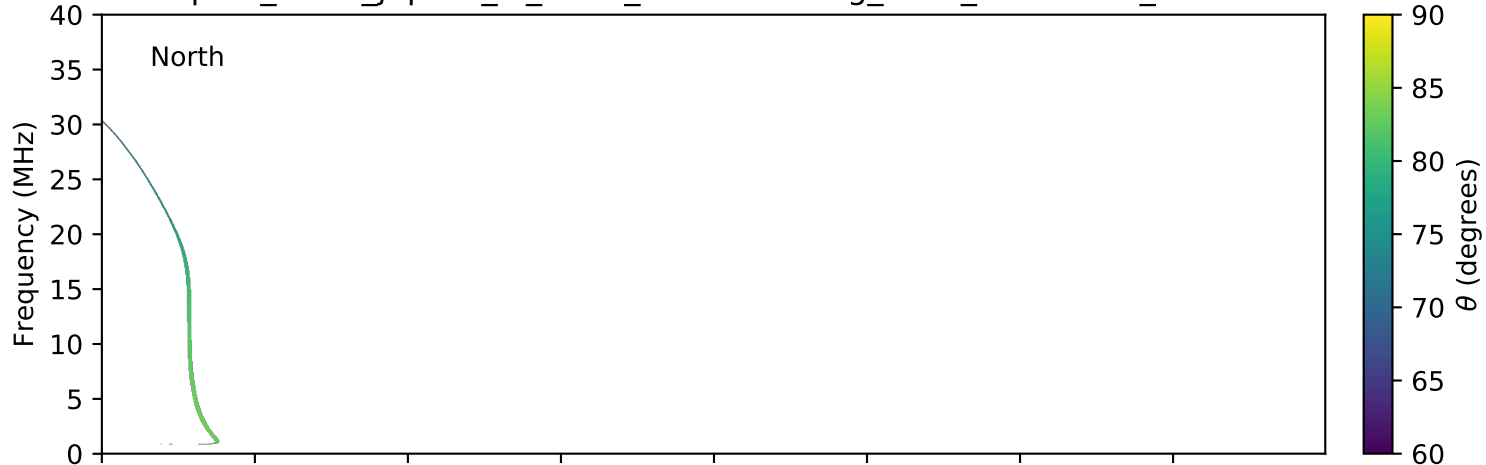
expres_earth_jupiter_io_isaac_lossc-wid1deg_3kev_20051224_v01.cdf
