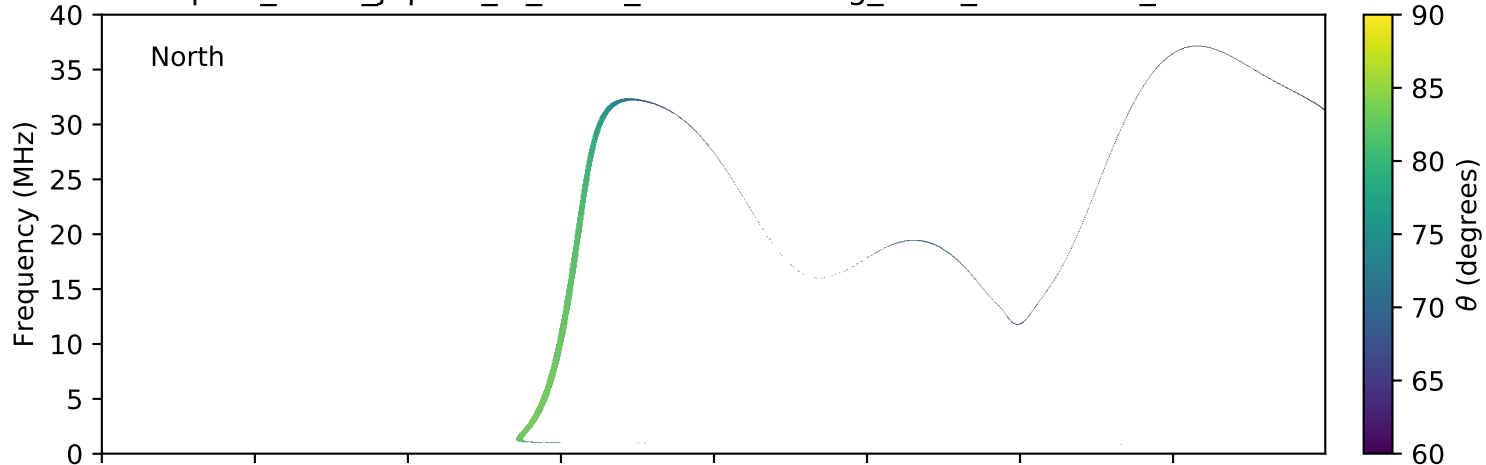
expres_earth_jupiter_io_isaac_lossc-wid1deg_3kev_20051223_v01.cdf
