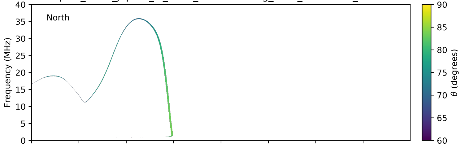
expres_earth_jupiter_io_isaac_lossc-wid1deg_3kev_20051222_v01.cdf
