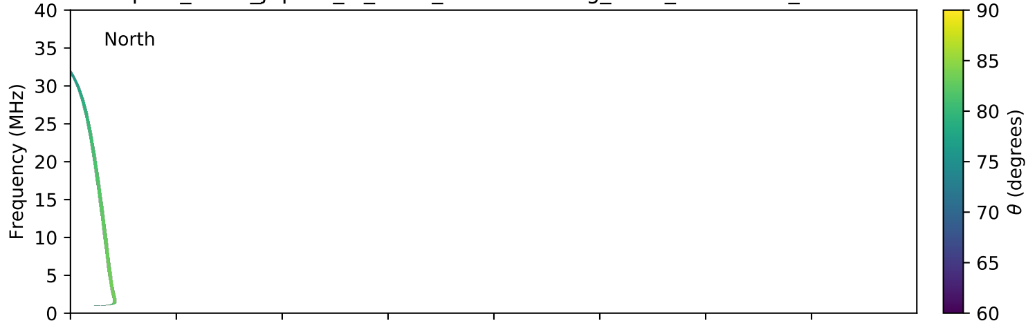
expres_earth_jupiter_io_isaac_lossc-wid1deg_3kev_20051217_v01.cdf
