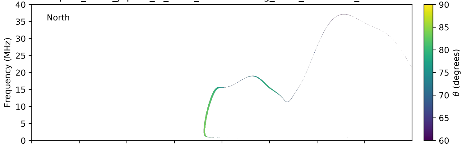
expres_earth_jupiter_io_isaac_lossc-wid1deg_3kev_20051214_v01.cdf
