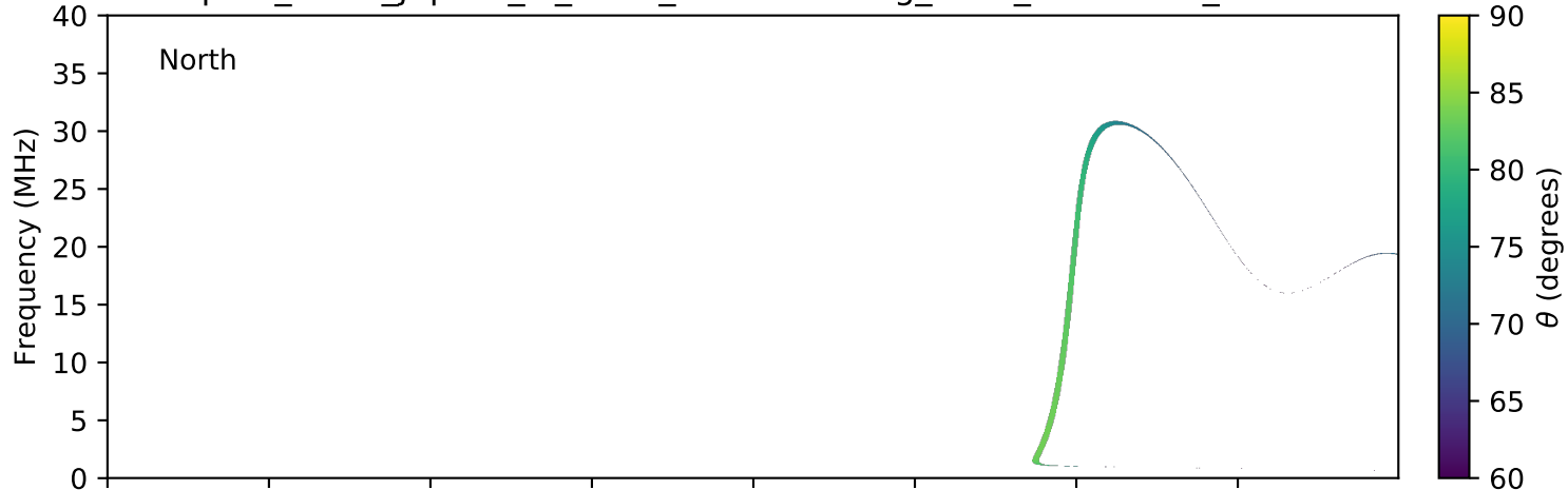
expres_earth_jupiter_io_isaac_lossc-wid1deg_3kev_20051212_v01.cdf
