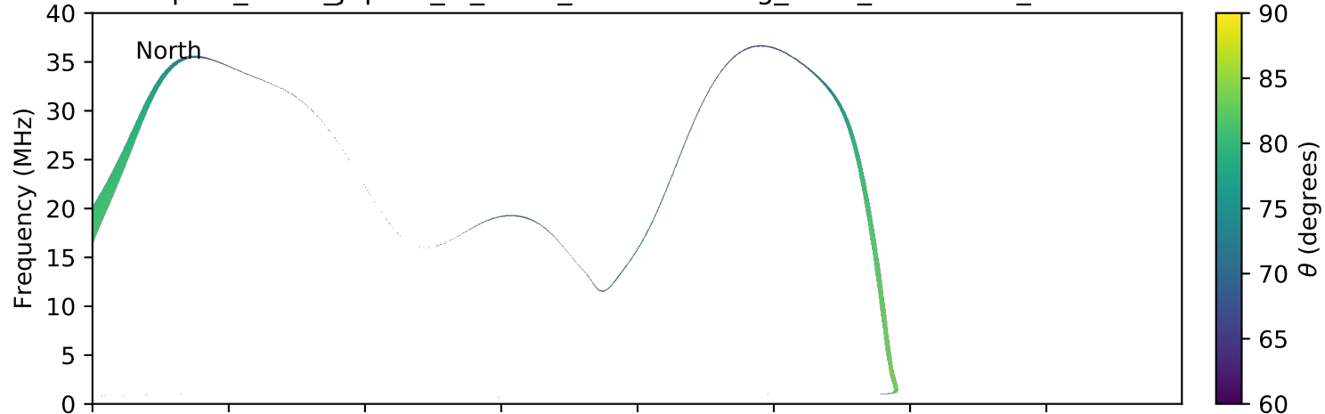
expres_earth_jupiter_io_isaac_lossc-wid1deg_3kev_20051211_v01.cdf
