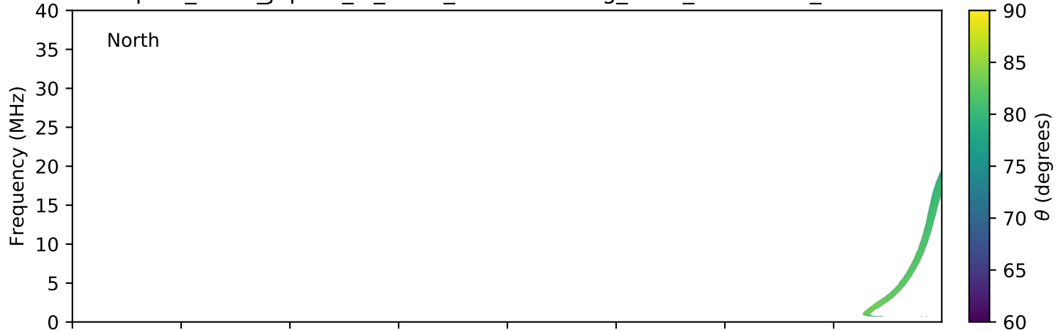
expres_earth_jupiter_io_isaac_lossc-wid1deg_3kev_20051210_v01.cdf
