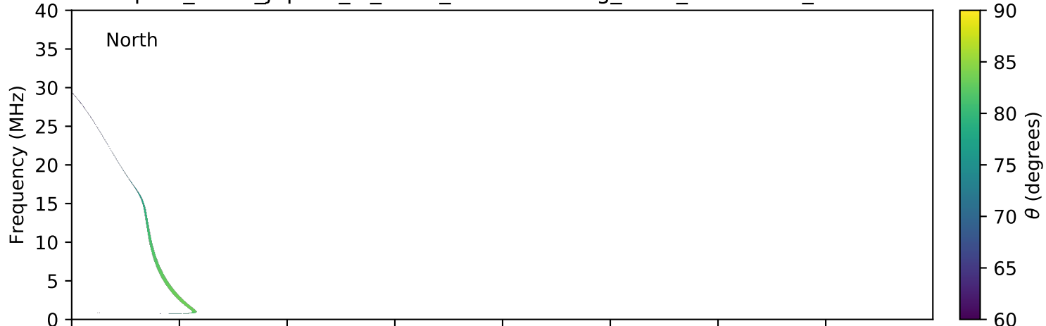
expres_earth_jupiter_io_isaac_lossc-wid1deg_3kev_20051208_v01.cdf
