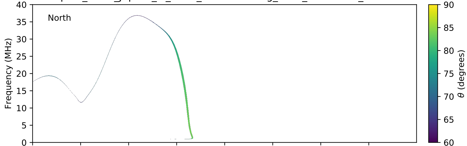
expres_earth_jupiter_io_isaac_lossc-wid1deg_3kev_20051206_v01.cdf
