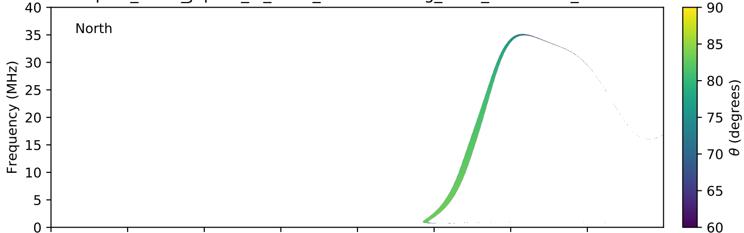
expres_earth_jupiter_io_isaac_lossc-wid1deg_3kev_20051205_v01.cdf
