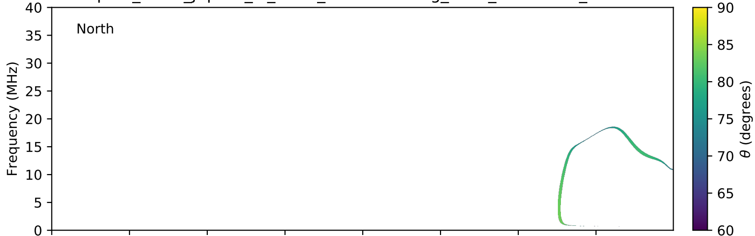
expres_earth_jupiter_io_isaac_lossc-wid1deg_3kev_20051203_v01.cdf
