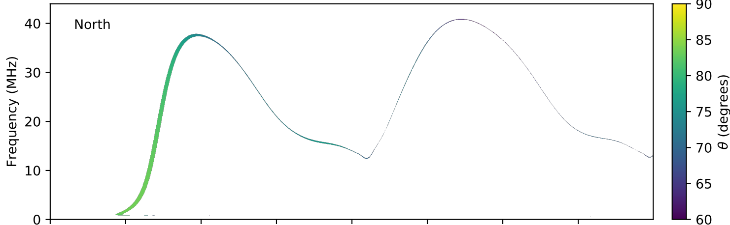
expres_earth_jupiter_europa_jrm09_lossc-wid1deg_3kev_20051222_v01.cdf
