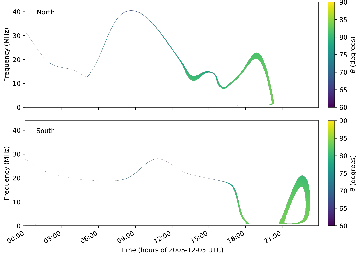
expres_earth_jupiter_europa_jrm09_lossc-wid1deg_3kev_20051205_v01.cdf
