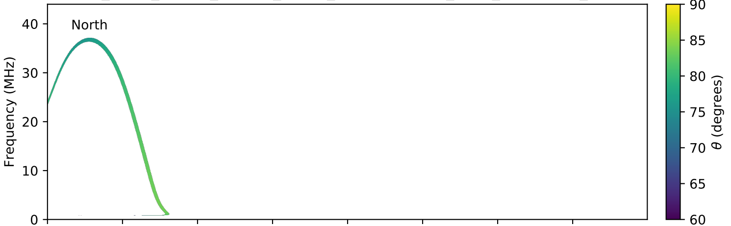
expres_earth_jupiter_europa_jrm09_lossc-wid1deg_3kev_20051202_v01.cdf
