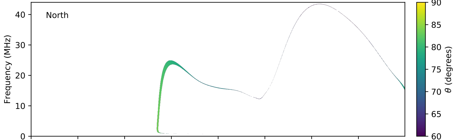
expres_earth_jupiter_io_jrm09_lossc-wid1deg_3kev_20051130_v01.cdf
