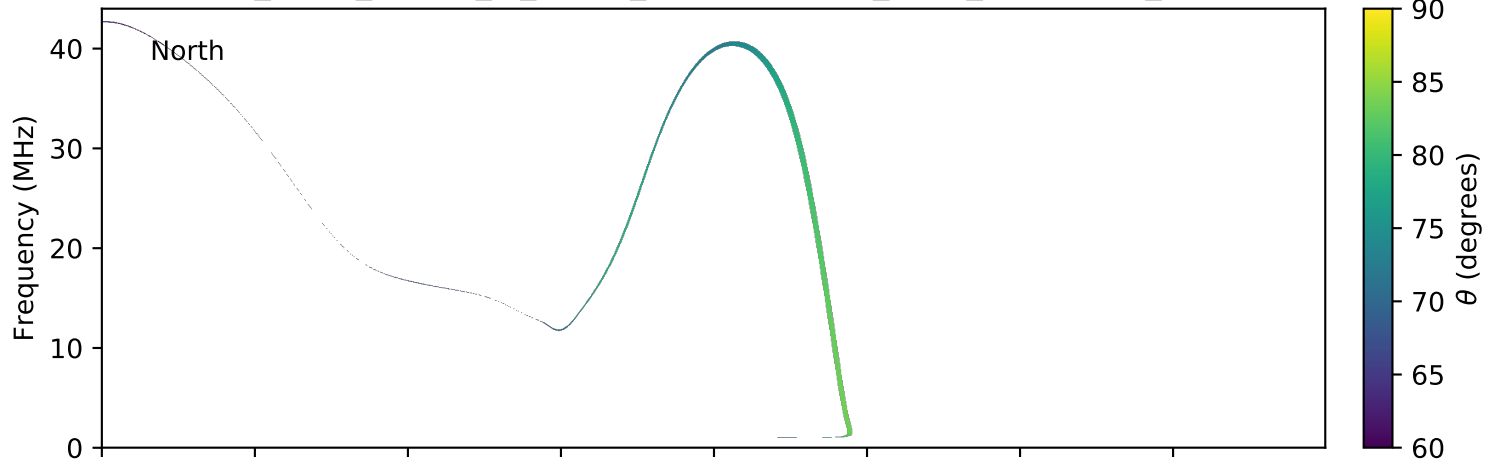
expres_earth_jupiter_io_jrm09_lossc-wid1deg_3kev_20051127_v01.cdf
