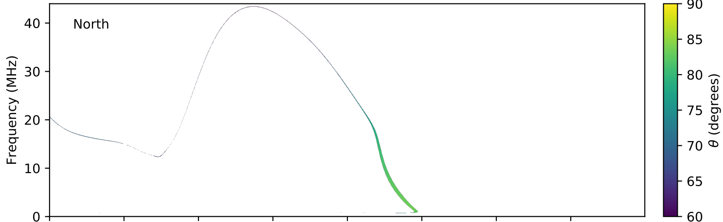
expres_earth_jupiter_io_jrm09_lossc-wid1deg_3kev_20051111_v01.cdf
