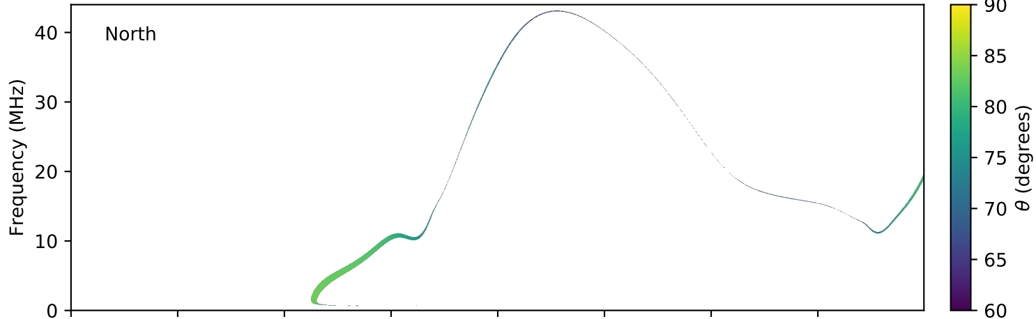
expres_earth_jupiter_io_jrm09_lossc-wid1deg_3kev_20051107_v01.cdf
