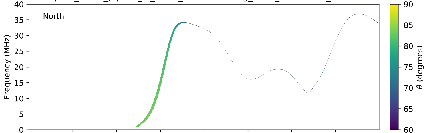
expres_earth_jupiter_io_isaac_lossc-wid1deg_3kev_20051130_v01.cdf
