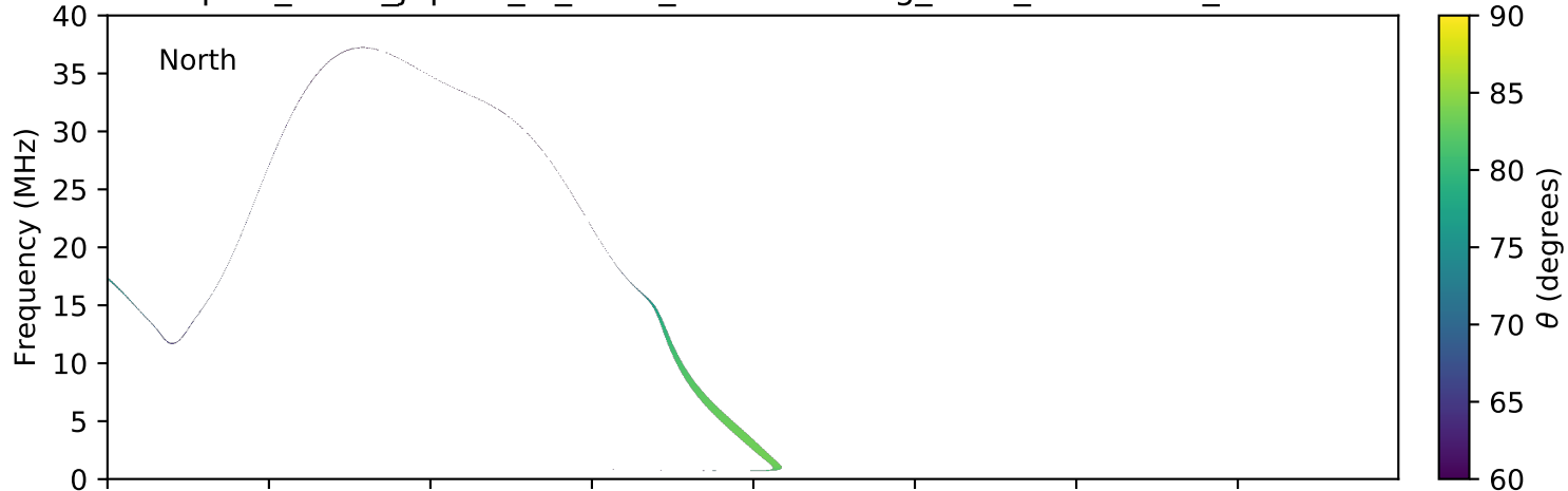
expres_earth_jupiter_io_isaac_lossc-wid1deg_3kev_20051127_v01.cdf
