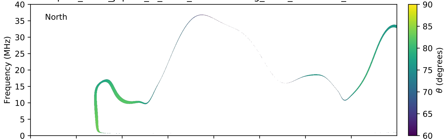
expres_earth_jupiter_io_isaac_lossc-wid1deg_3kev_20051123_v01.cdf
