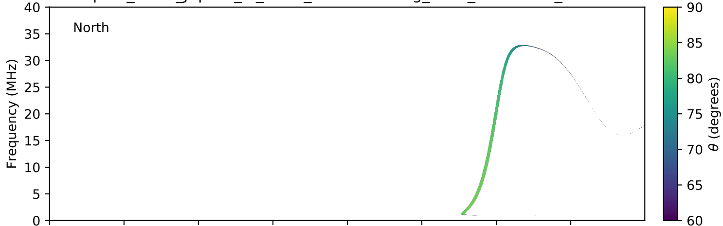
expres_earth_jupiter_io_isaac_lossc-wid1deg_3kev_20051119_v01.cdf
