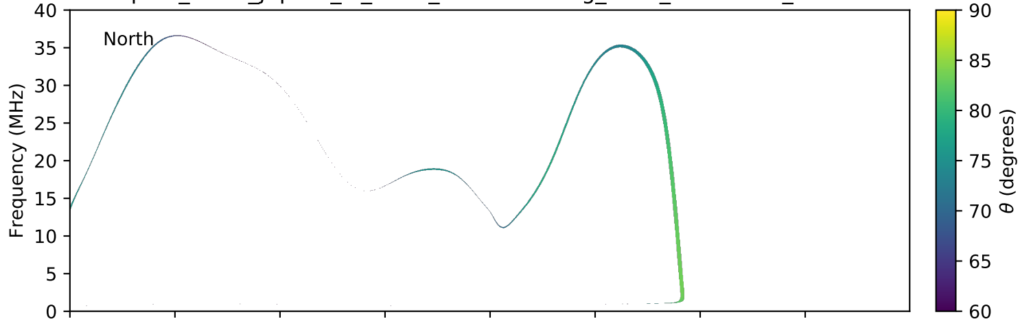
expres_earth_jupiter_io_isaac_lossc-wid1deg_3kev_20051118_v01.cdf
