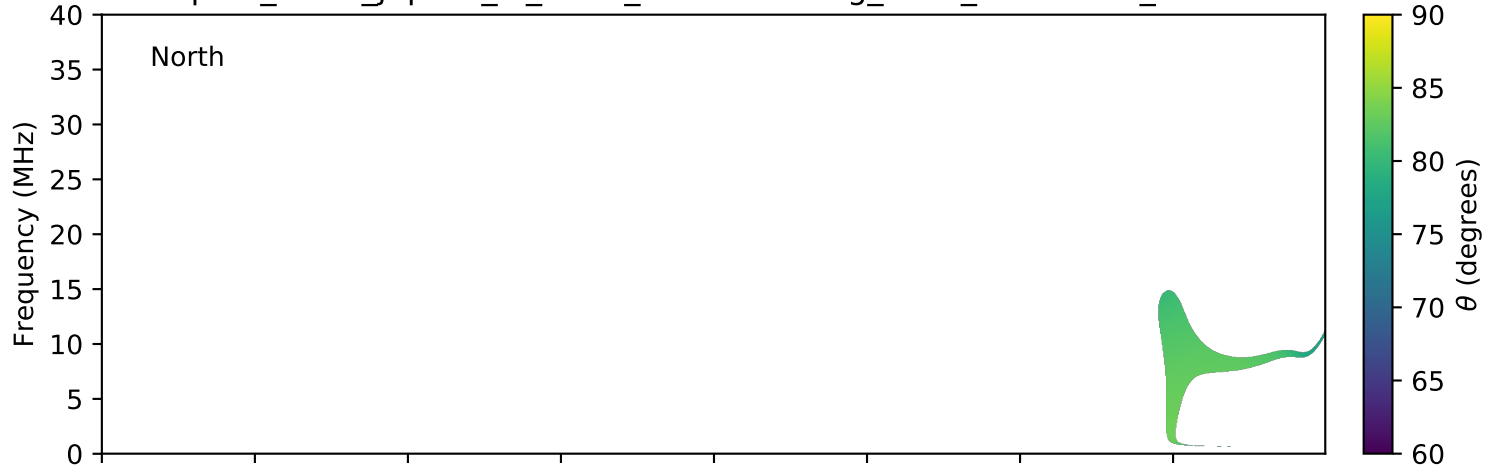
expres_earth_jupiter_io_isaac_lossc-wid1deg_3kev_20051117_v01.cdf
