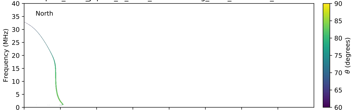
expres_earth_jupiter_io_isaac_lossc-wid1deg_3kev_20051115_v01.cdf
