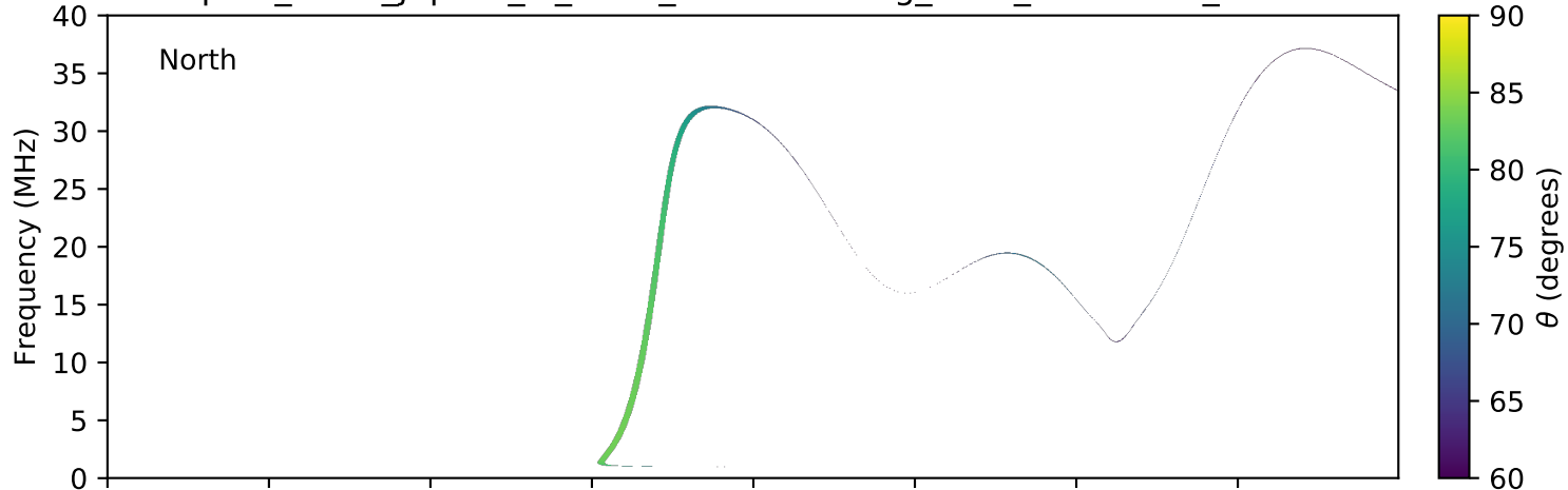
expres_earth_jupiter_io_isaac_lossc-wid1deg_3kev_20051114_v01.cdf
