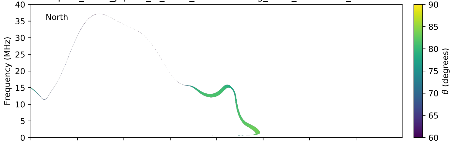
expres_earth_jupiter_io_isaac_lossc-wid1deg_3kev_20051111_v01.cdf
