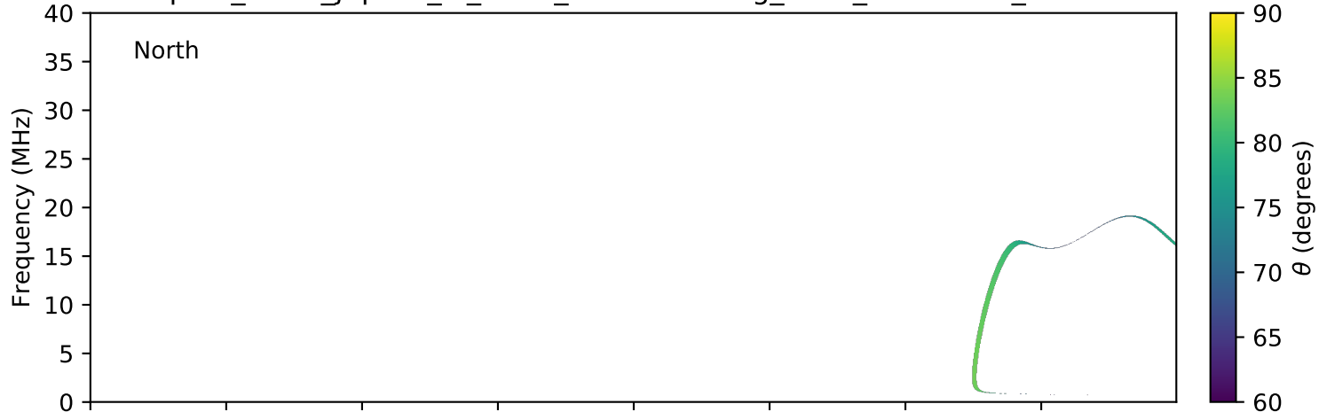
expres_earth_jupiter_io_isaac_lossc-wid1deg_3kev_20051110_v01.cdf
