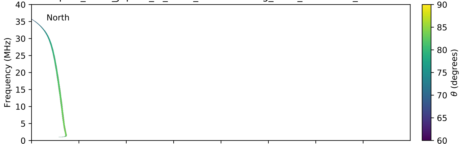
expres_earth_jupiter_io_isaac_lossc-wid1deg_3kev_20051108_v01.cdf
