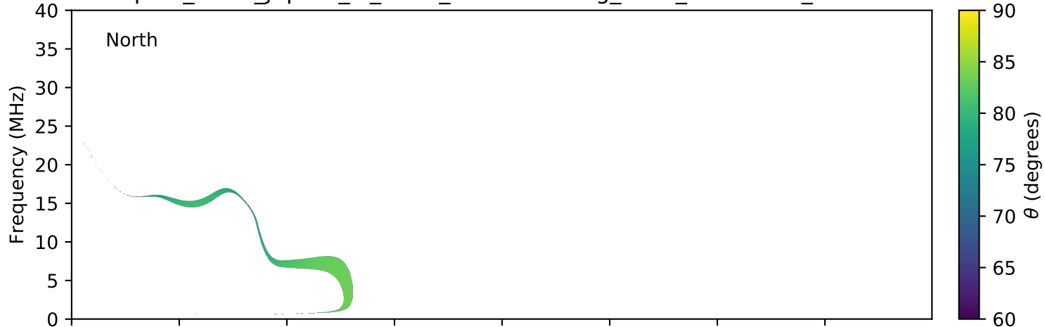
expres_earth_jupiter_io_isaac_lossc-wid1deg_3kev_20051106_v01.cdf
