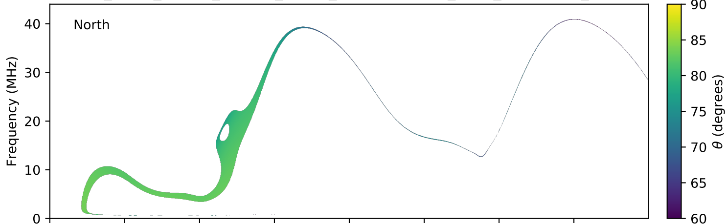
expres_earth_jupiter_europa_jrm09_lossc-wid1deg_3kev_20051127_v01.cdf
