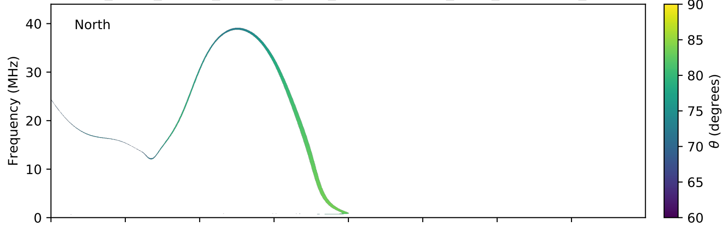
expres_earth_jupiter_europa_jrm09_lossc-wid1deg_3kev_20051121_v01.cdf
