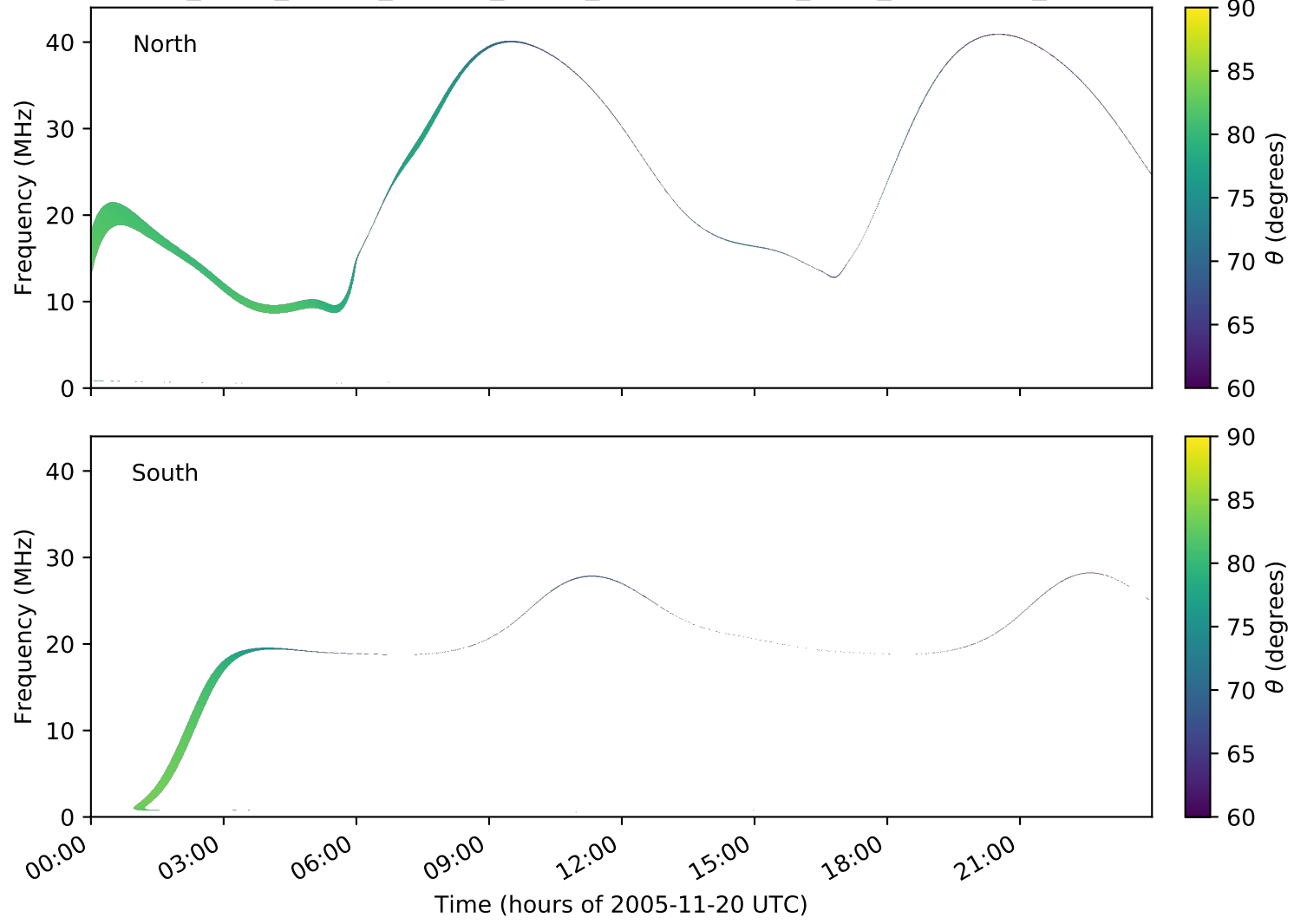
expres_earth_jupiter_europa_jrm09_lossc-wid1deg_3kev_20051120_v01.cdf
