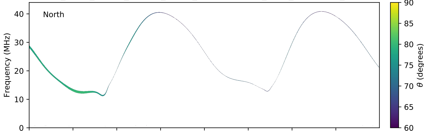
expres_earth_jupiter_europa_jrm09_lossc-wid1deg_3kev_20051113_v01.cdf
