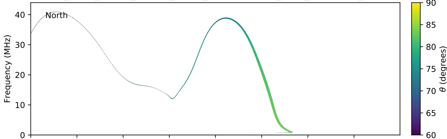
expres_earth_jupiter_europa_jrm09_lossc-wid1deg_3kev_20051103_v01.cdf
