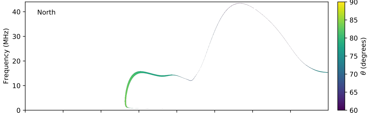
expres_earth_jupiter_io_jrm09_lossc-wid1deg_3kev_20050929_v01.cdf
